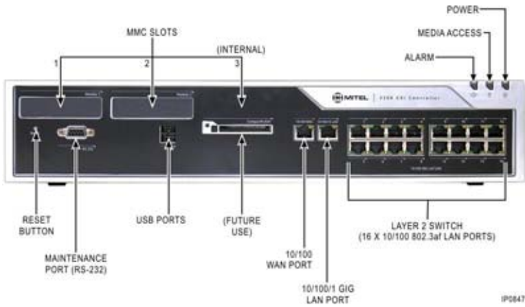
Figure 99: CXi Controller – Front Panel
