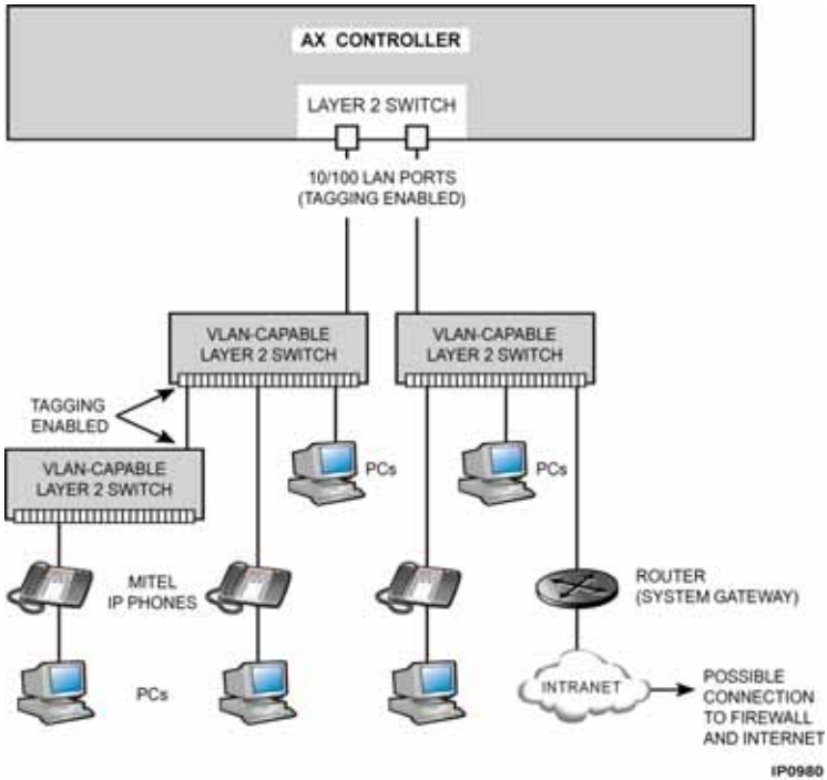
Figure 128: AX Voice and Data Configuration Example
