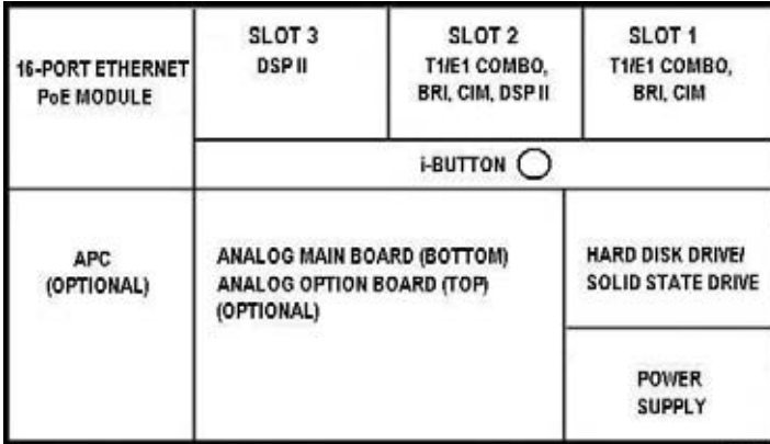
Figure 9: Slot Locations for the CXi II Controller (with an Ethernet L2 Switch with POE)
