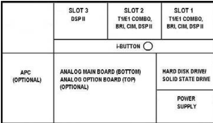
Figure 10: Slot Locations for the CX II Controller (without an Ethernet L2 Switch)
