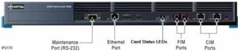
Figure 109: Universal NSU – Front Panel
