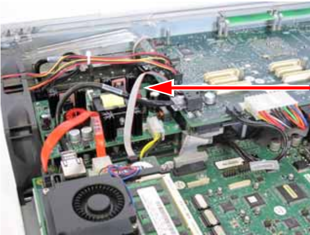
Figure 65: Cable Routing
