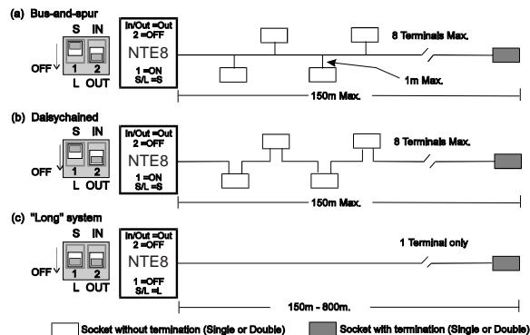
Diagram 1 – ISDN Extensions
